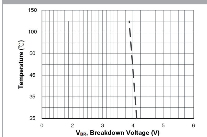
Fig6. Typical Breakdown Voltage vs. Temperature
