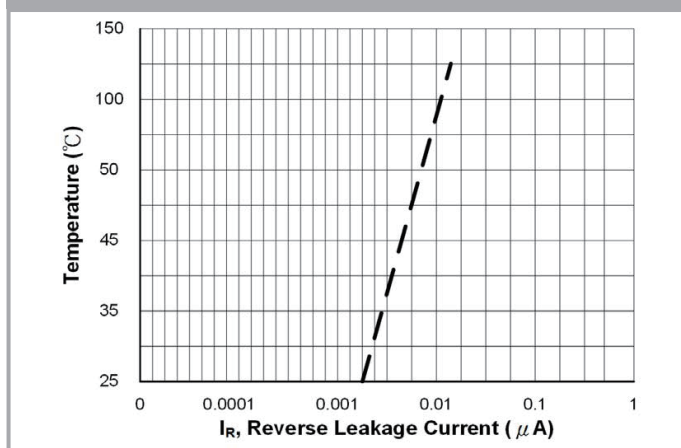
Fig4. Typical Reverse Leakage vs. Temperature
