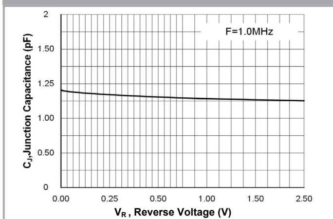
Fig5. Typical Capacitance vs. Reverse Voltage
